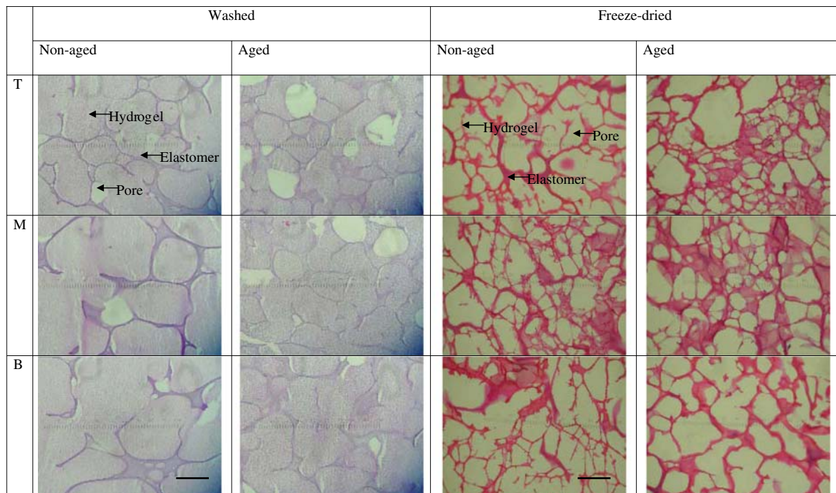
Fig. 1 Typical light microscopy photographs of IPN films prepared with either a fresh (i.e. non-aged) solution of methacrylated gelatin at 7.5 wt% or a solution aged at 7.5 wt% and room temperature for 3 weeks (i.e. aged). Films were sliced
