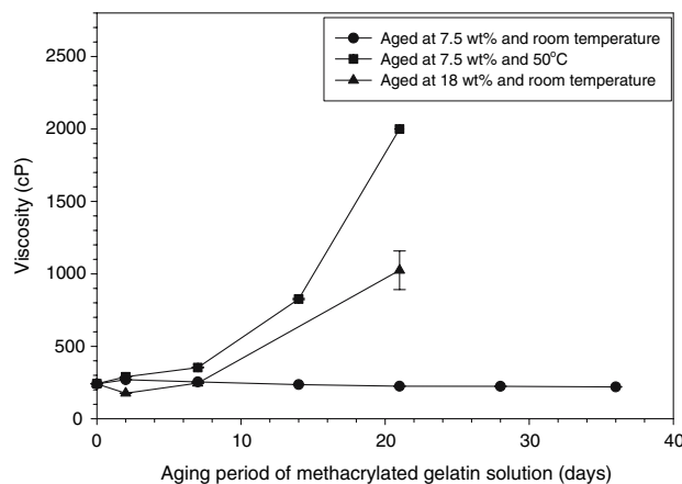
Fig. 6 Aging effects on the viscosity of methacrylated gelatin solutions. Methacrylated gelatin solutions were prepared at 7.5 and 18 wt% in DMSO and kept either at room temperature or 50°C for up to 36 days. Data represent means \pm standard deviation ( n = 3 )
